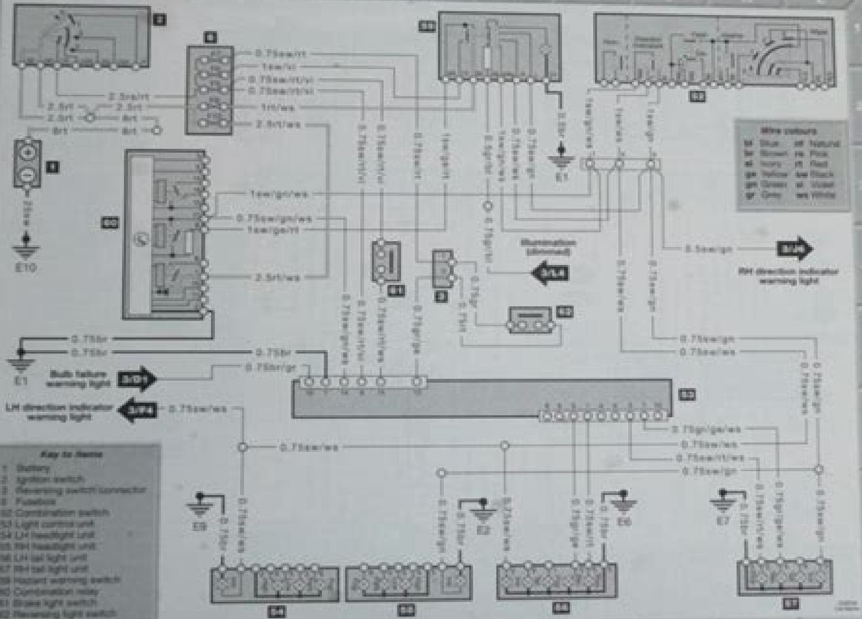
Diagram 5: Exterior lighting continued - direction indicators, hazard warning, stop and reversing lights
