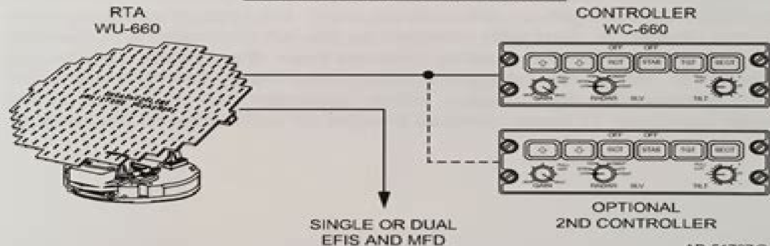
PRIMUS® 660 Configurations Figure 2-1
