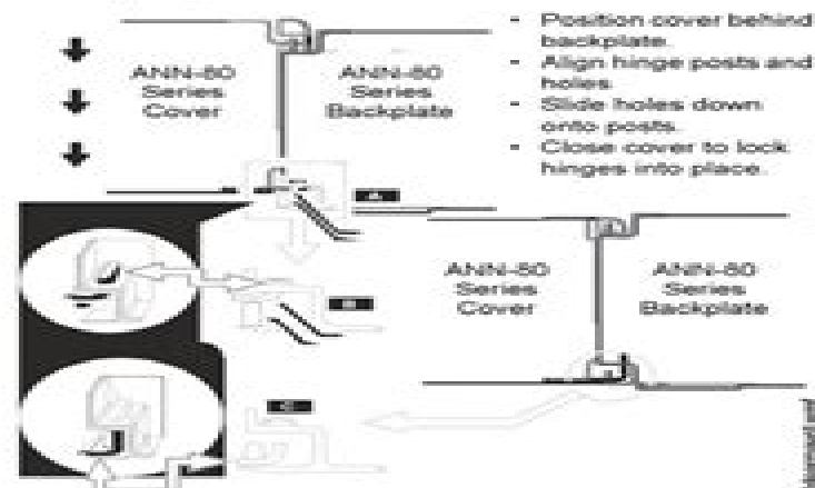
Figure 2 Cover Reattachment
