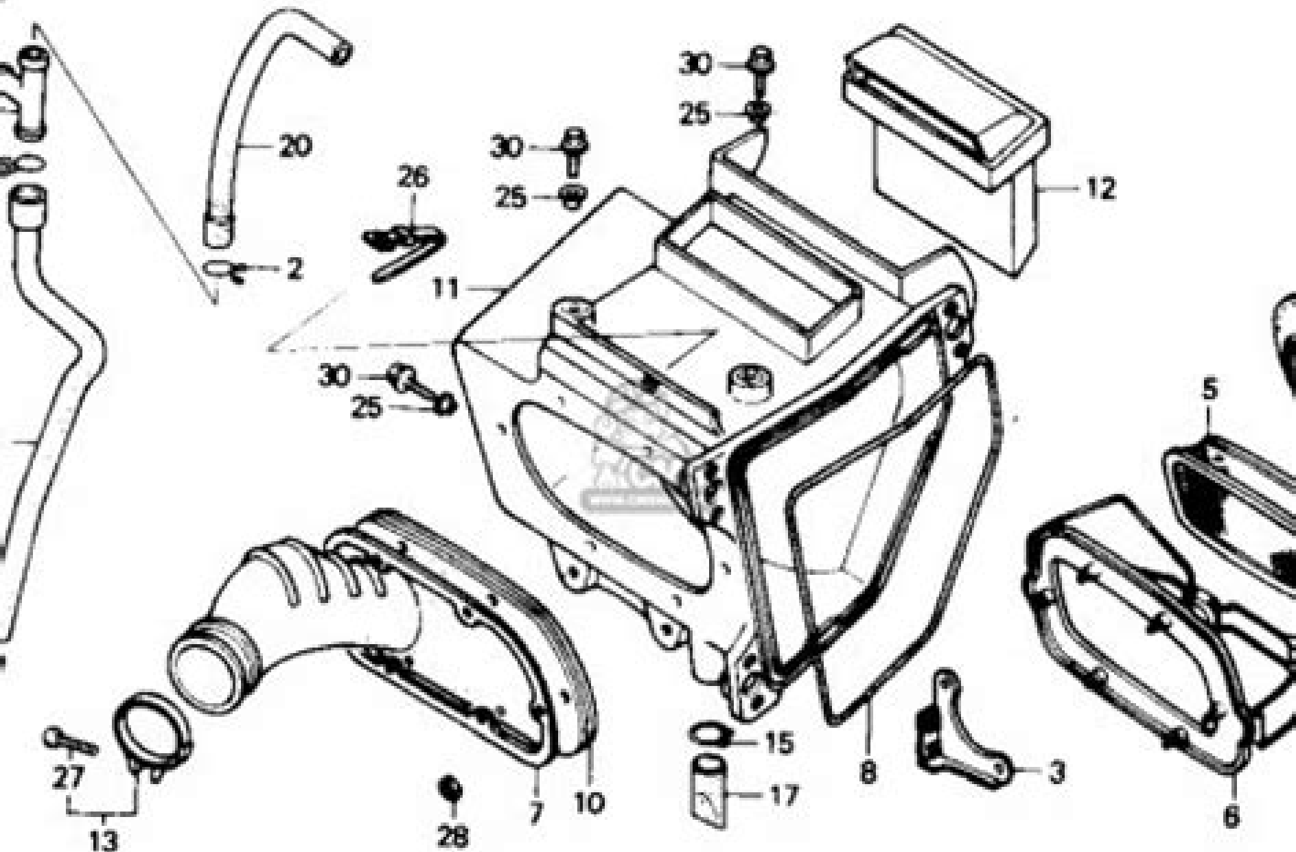
AIR CLEANER 86-91
