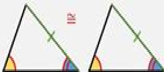
AAS Angle-Angle-Side
