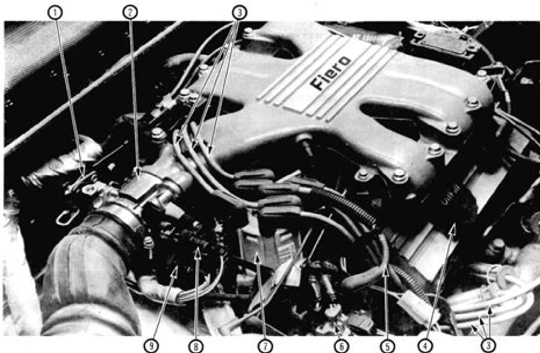
The engine compartment of a Fiero with a 2.8L V6 engine (viewed from the left side)
