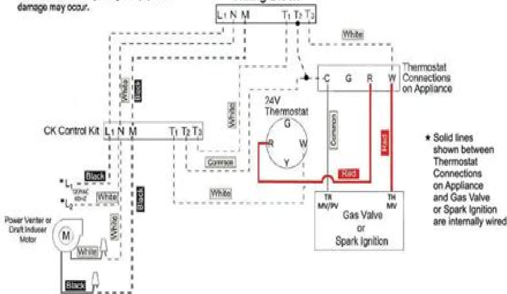
Diagram F - Power Vent Single 24V Furnace
