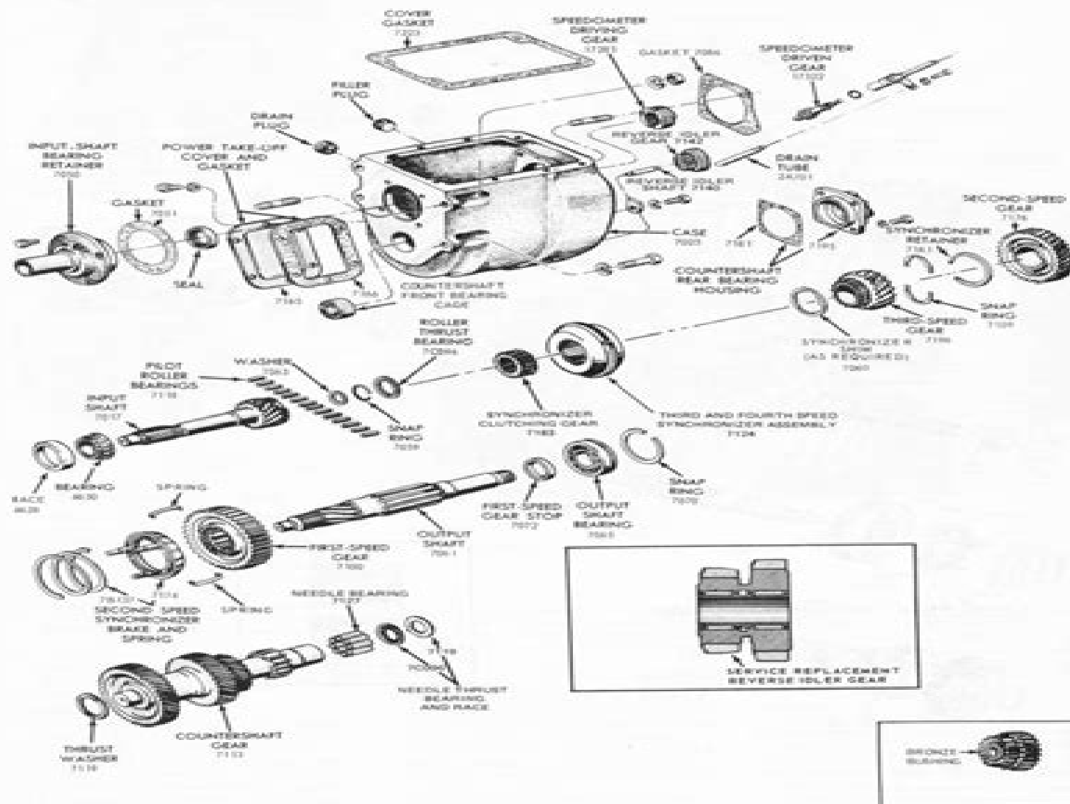
FIG. 5 Transmission Disassembled—F-100-F-350, F-600, Bronco
