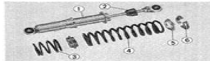
Fig. 2-46 ① Rear damper ② Stopper rubber ③ Rear cushion spring A ④ Rear cushion spring B ⑤ Rear cushion spring seat ⑥ Spring seat stopper
