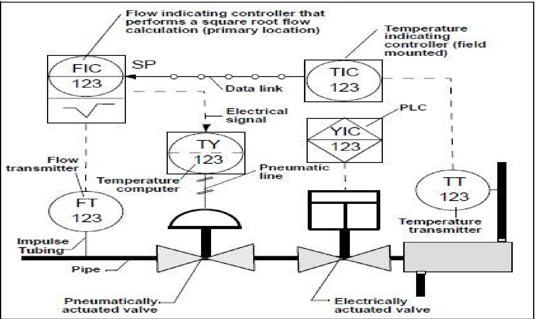
P&ID with ISA Symbology
