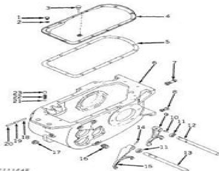
Fig. 2-Transmission and Differential Case (160,001- )
