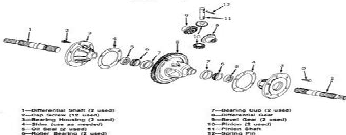
Fig. 3-Differential Assembly
