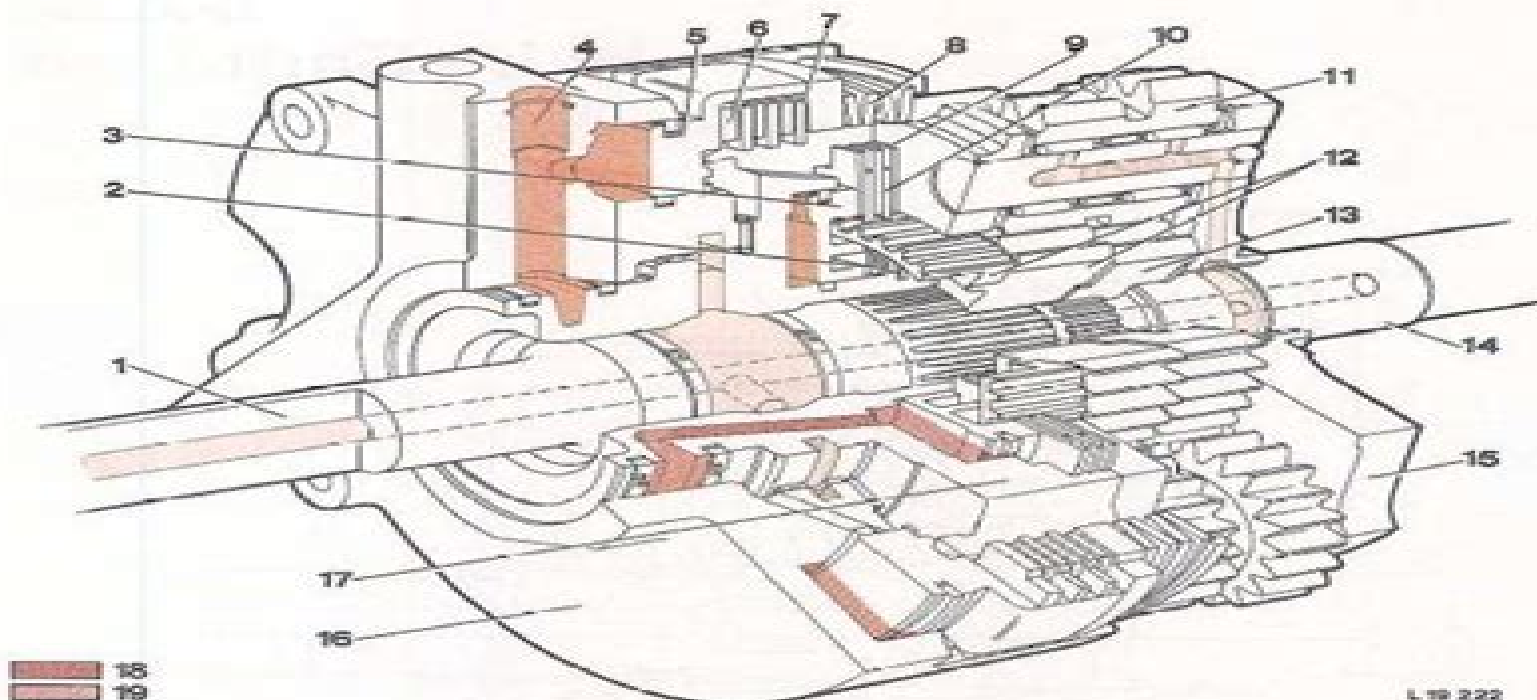
Fig. 2 – Hi-Lo Shift Unit, Oil Flow
