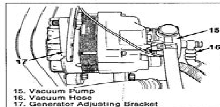
Figure 6. Vacuum Hose Attachment at Vacuum Pump
