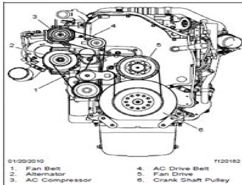
Fig. 1, Cummins ISX Drive Belt Routing
