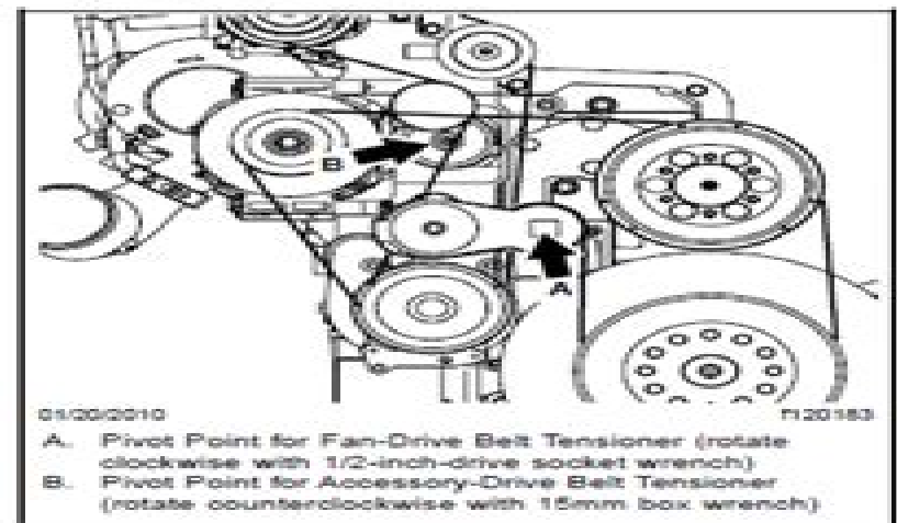
Fig. 2, Releasing the Tensioners
