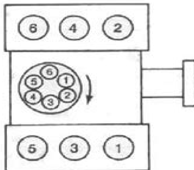
GM (Chevrolet) 173 V6 (2.8 L) Engine firing order: 1-2-3-4-5-6 Distributor rotation: clockwise
