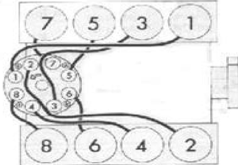
GM (Oldsmobile) 350, 403 V8 Engine firing order: 1-8-4-3-6-5-7-2 Distributor rotation: counterclockwise
