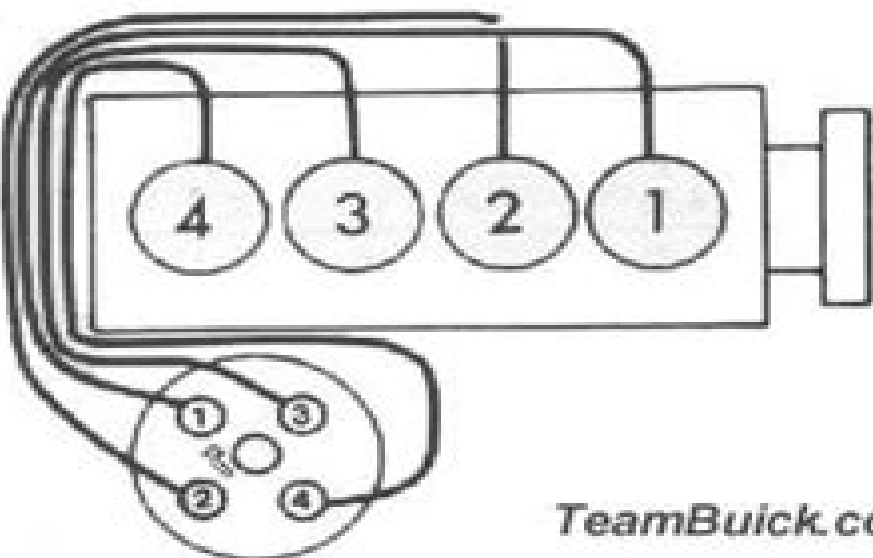
GM (Pontiac) 151-4 Engine firing order: 1-3-4-2 Distributor rotation: clockwise
