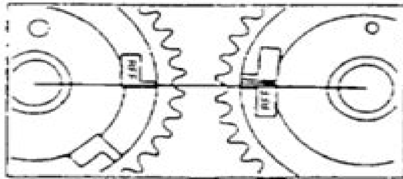
CAMSHAFT SPROCKET BACK SIDE
