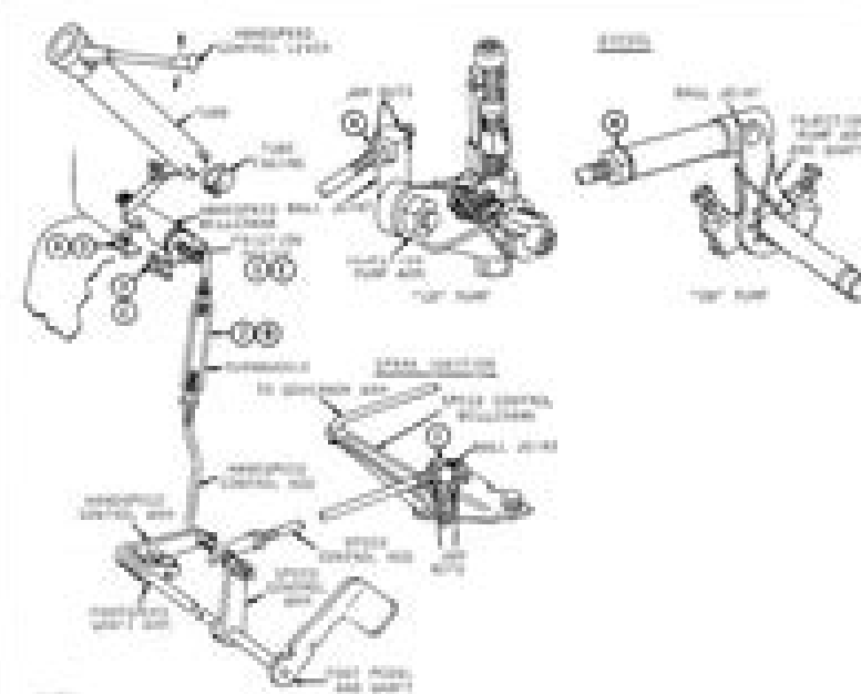
Fig. 11-Speed Control Linkage Installation and Adjustment
