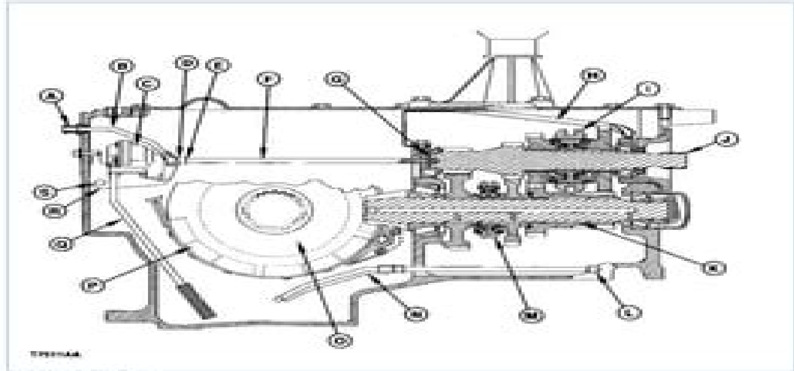
FIGURE 1-100 Transmission Diagram
