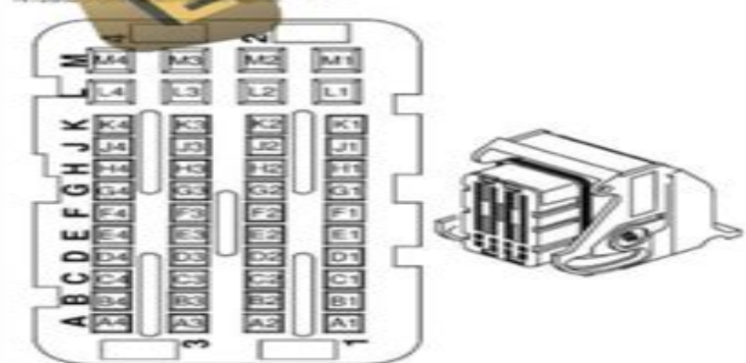
A8-605-UN: End View
