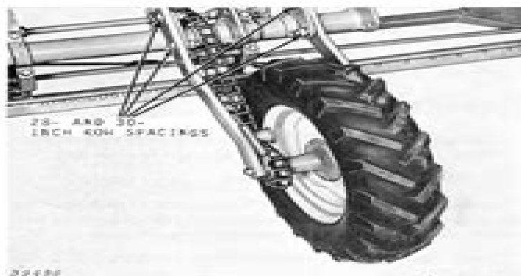
Wheel Setting for 28-through 30-inch Row Spacing
