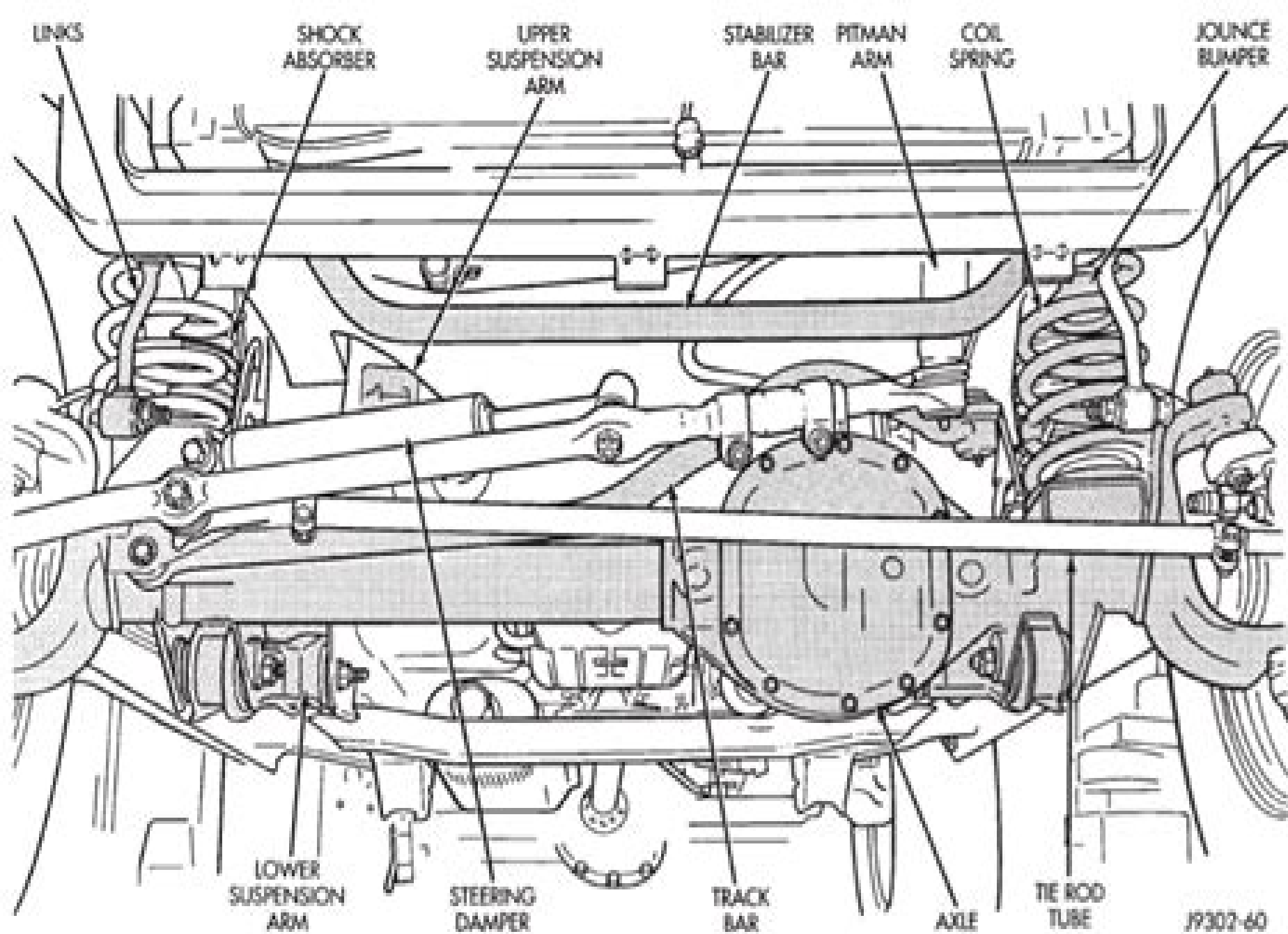
Fig. 1 Front Suspension (LHD)
