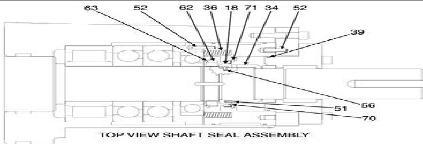
Figure 13a. Screw Compressor, TDSH 355.
