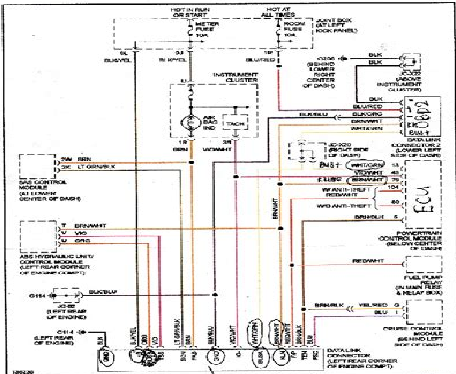
Fig. 8: Computer Data Lines
