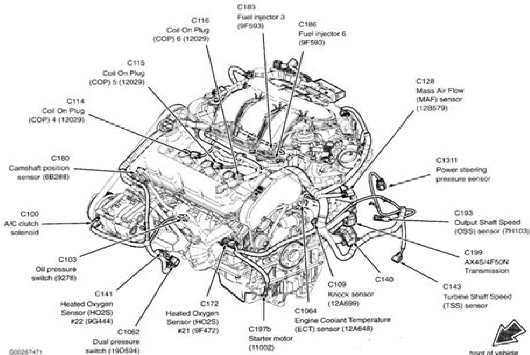
Fig 2: Front Of Engine (4V)
