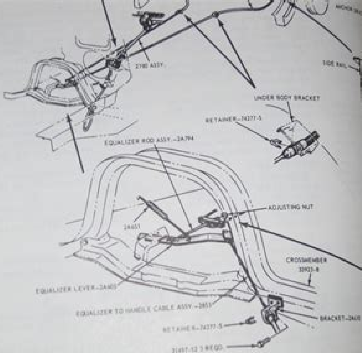
FIG. 27—Parking Brake Linkage—Mustang
