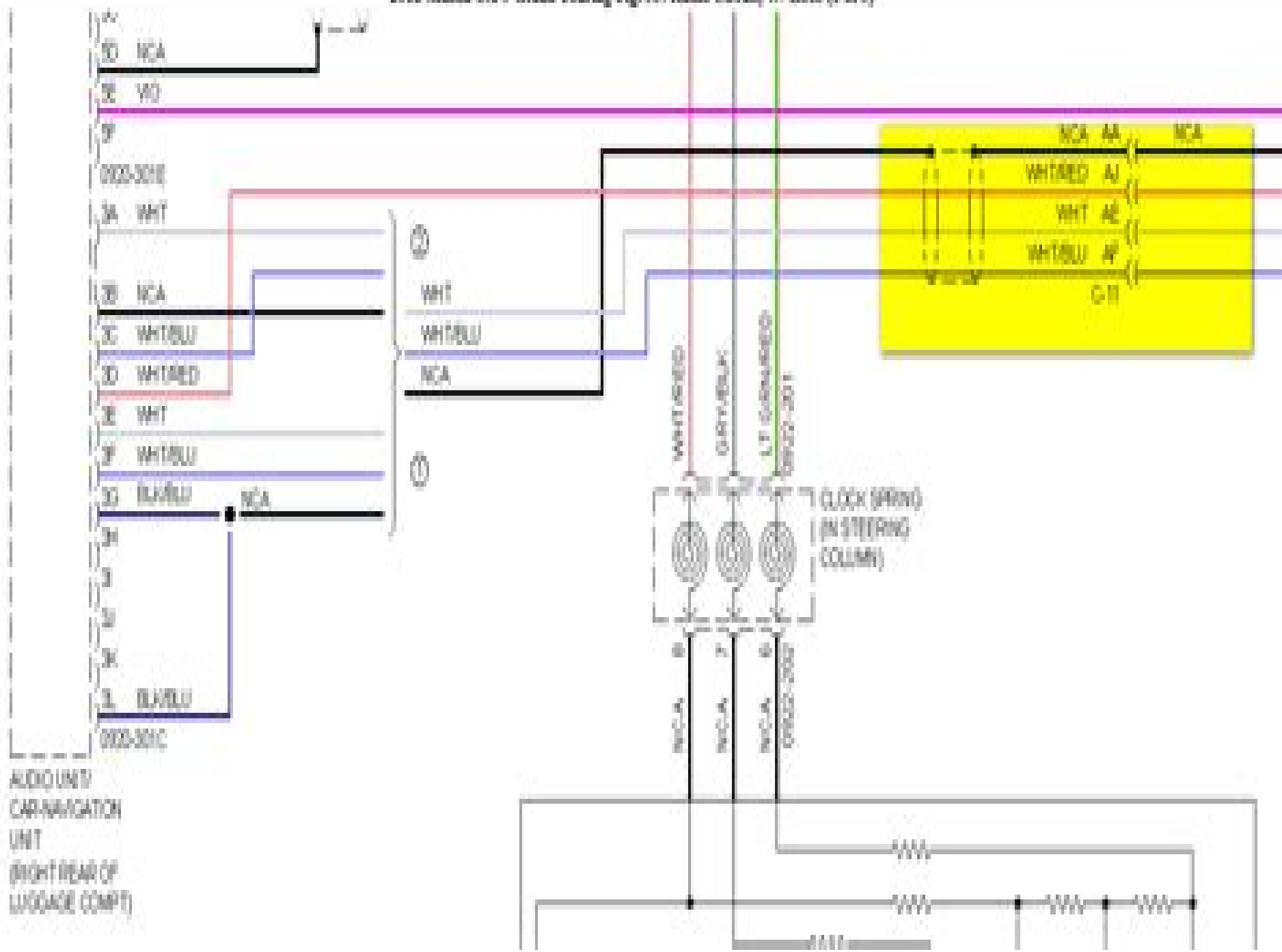
2012 Mazda CX-9 Grand Touring-Fig. 55: Radio Circuit, W/ Bose (1 of 3)
