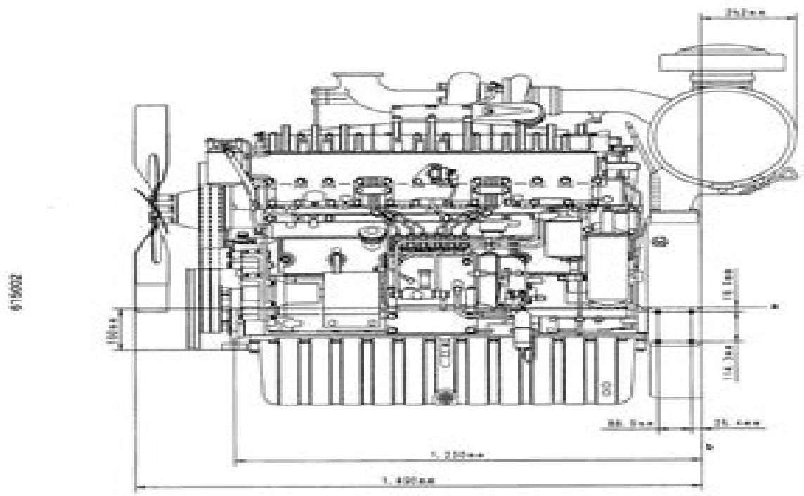
SA6D125-2 LEFT SIDE VIEW [For DCAJ3005SK (DENYO generator)]
