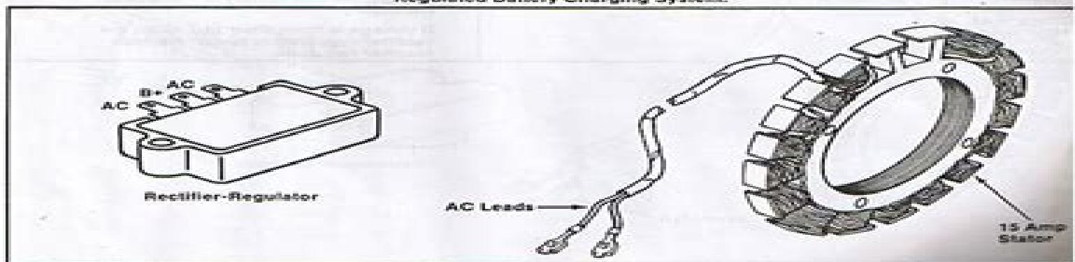
Figure 8-14. 15 Amp Stator And Rectifier-Regulator.
