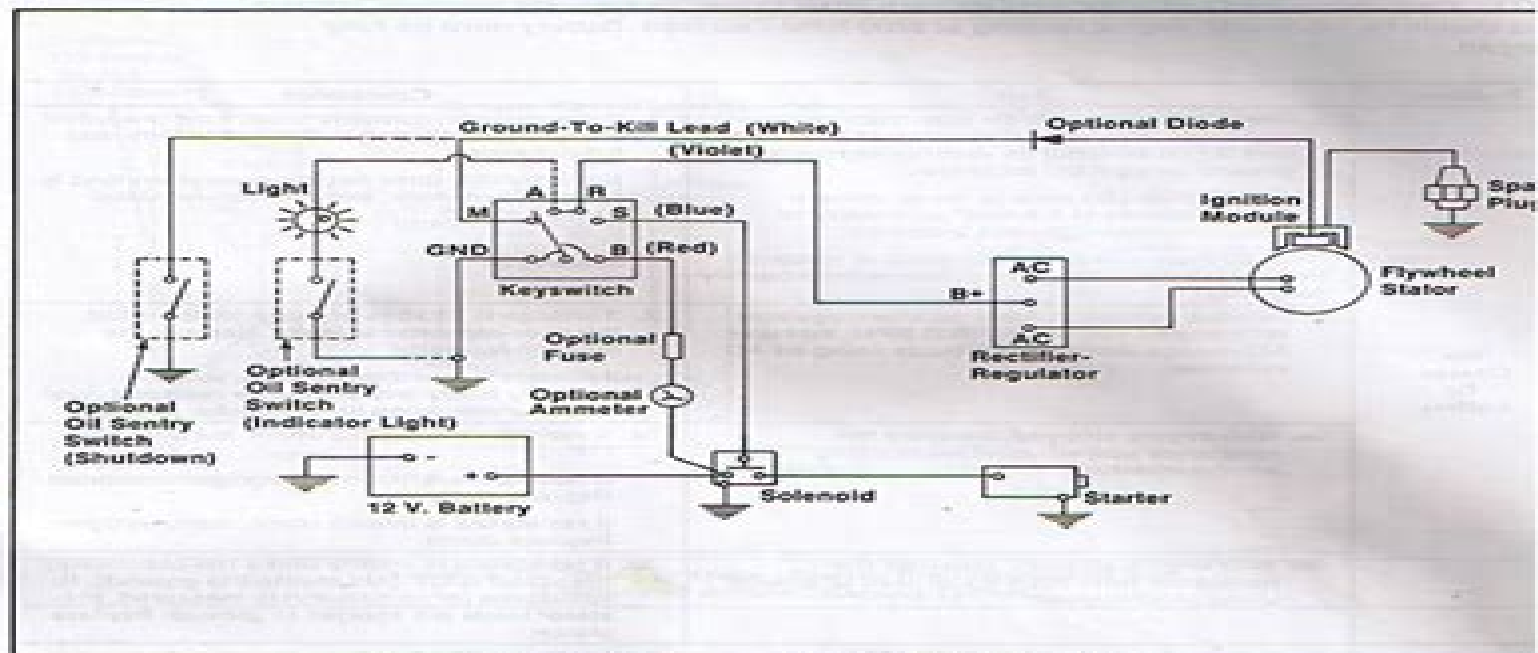
Figure 8-13. Wiring Diagram - Electric Start Engines/15 Amp Regulated Battery Charging System.
