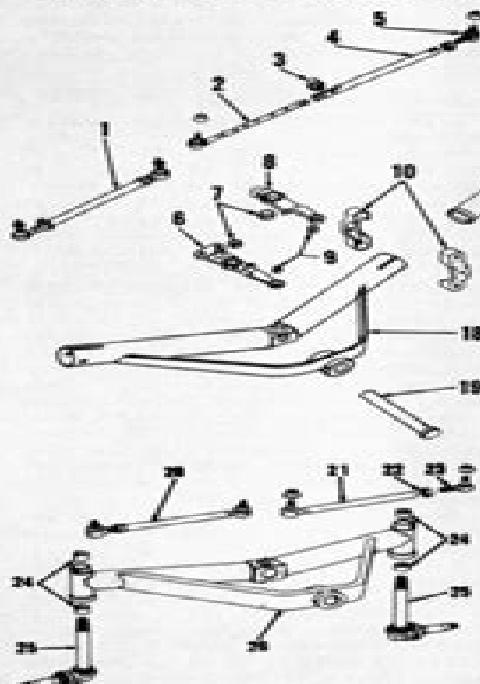
Fig. 7—Heavy duty non-adjustable front axle available for International 544 and 656 tractors. Refer to Fig. 8 for balance of components.
