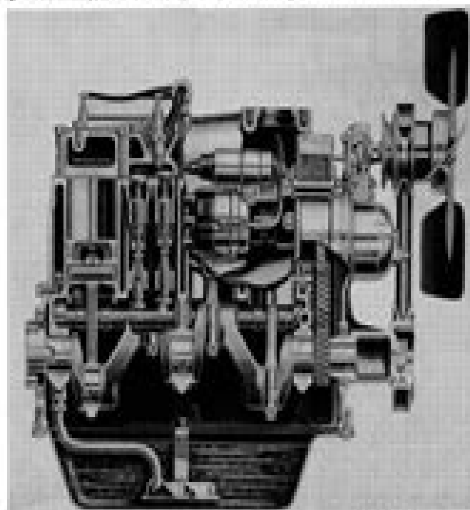
Fig. 1 - Basic section of Farmall Cub engine, side view
