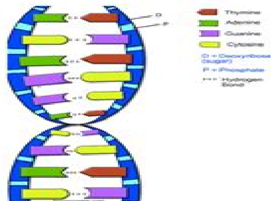
A simplified version of a DNA molecule.
