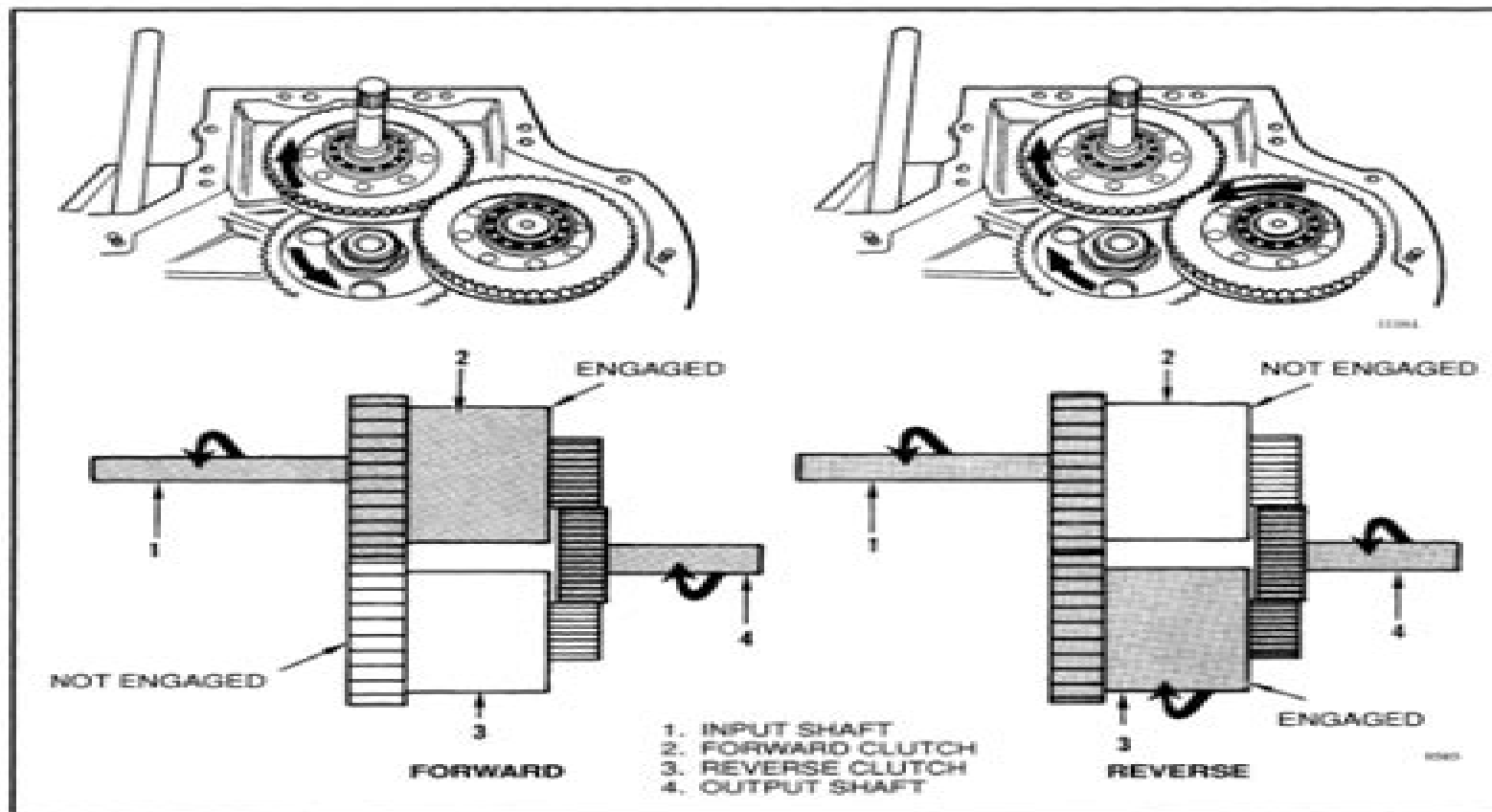
FIGURE 8. CLUTCH OPERATION
