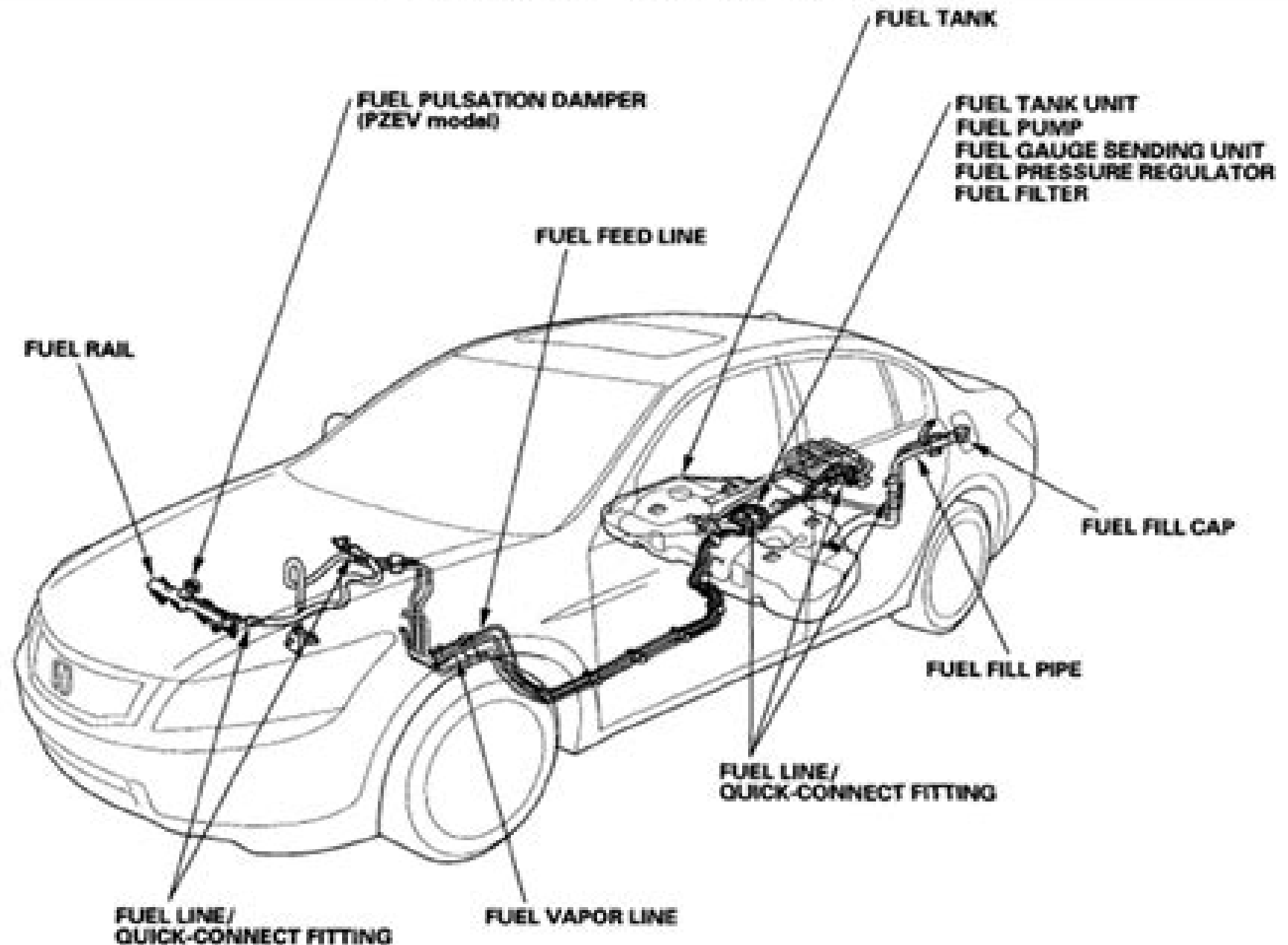
Fig. 1: Identifying Fuel Supply System Replacement Component Location (1 Of 2)
