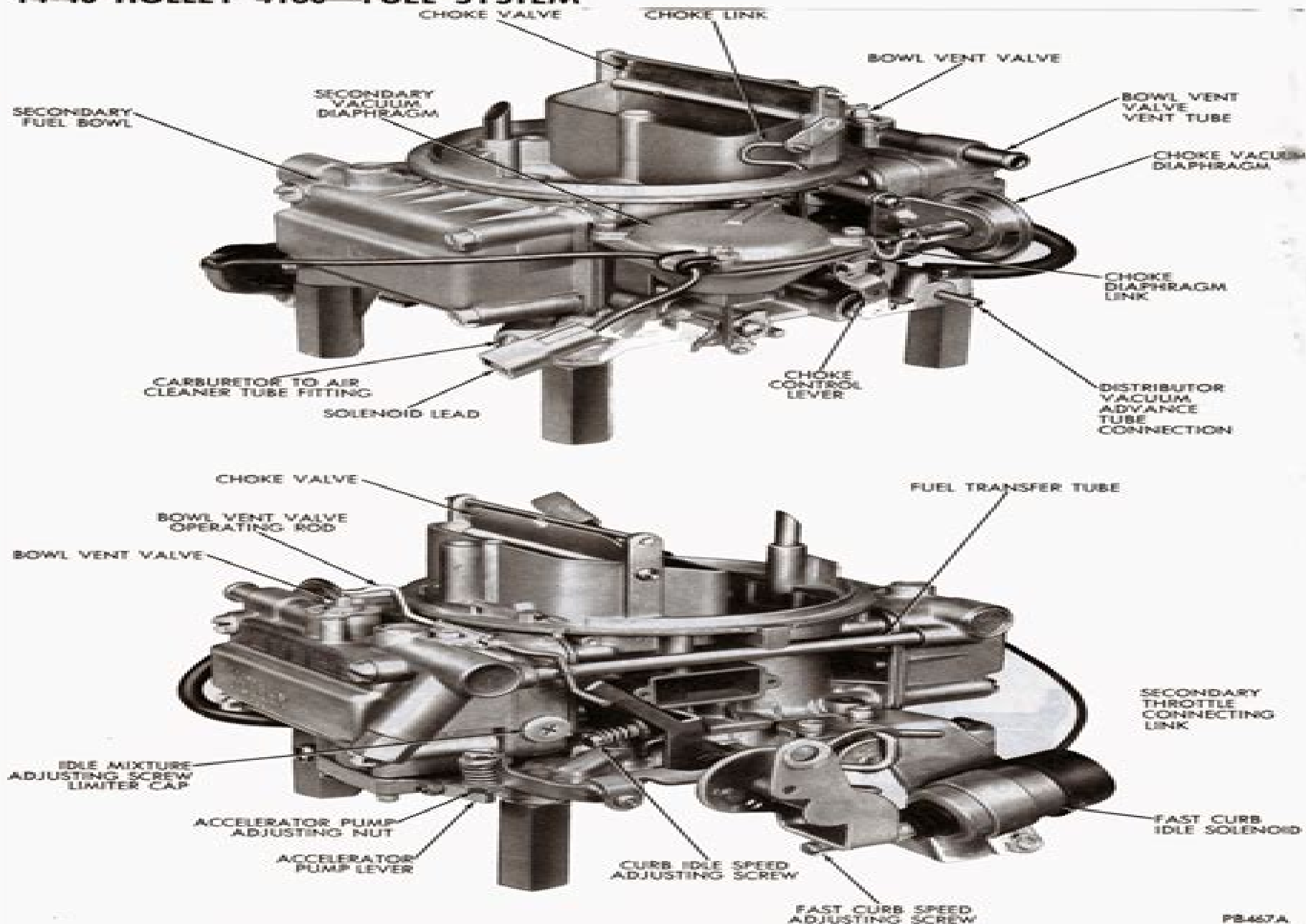
Fig. 2 - Carburetor Assembly - Holley Model 4160 (Manual Transmission)
