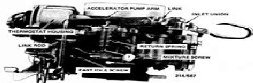
View of accelerator pump side of carburettor.
