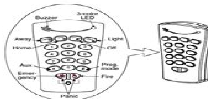
Figure 1 - External View
