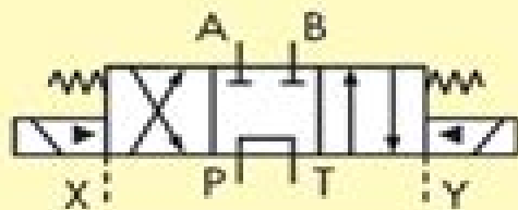
Directional Valves
