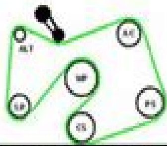
Bypassing the smog pump with A/C & P/S 84.5 Belt
