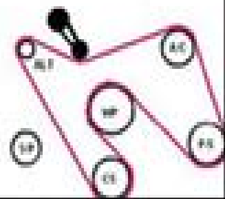
Bypassing the smog pump and using the Ford Racing M8511-A50 A/C Eliminator 73 Belt
