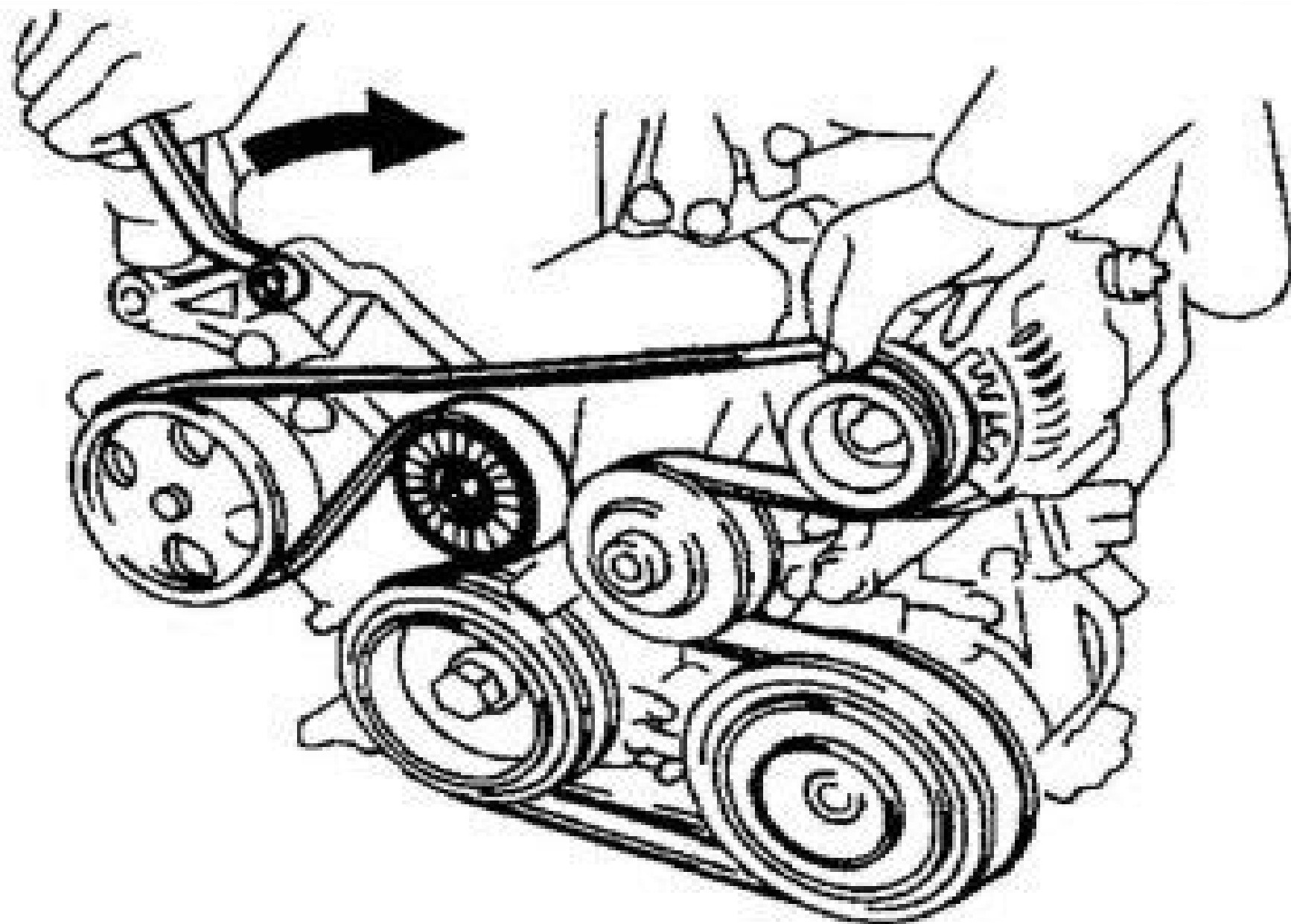
Fig. 440: Turning Drive Belt Tensioner Clockwise To Relieve Tension On Belt Courtesy of TOYOTA MOTOR SALES, U.S.A., INC.
