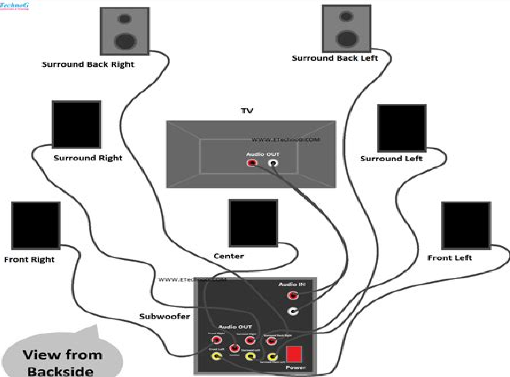
7.1 Home Theater Wiring and Connection Diagram
