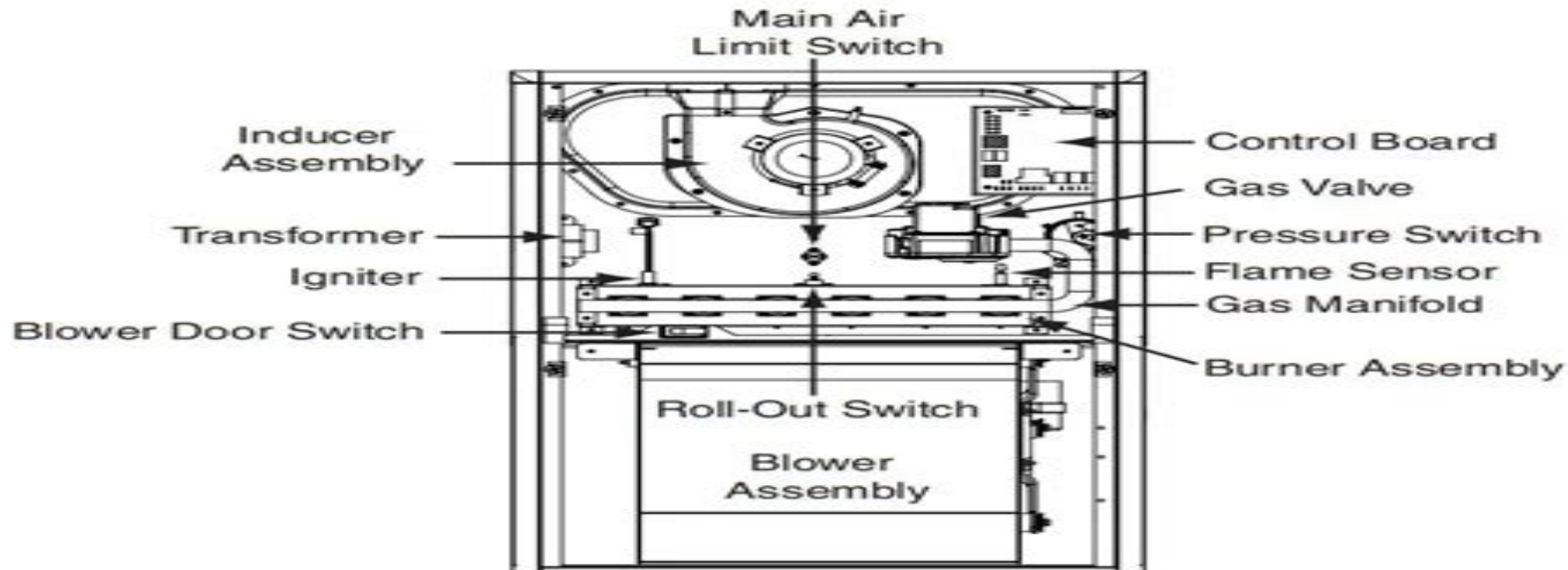
Upflow/Horizontal Gas Furnace
