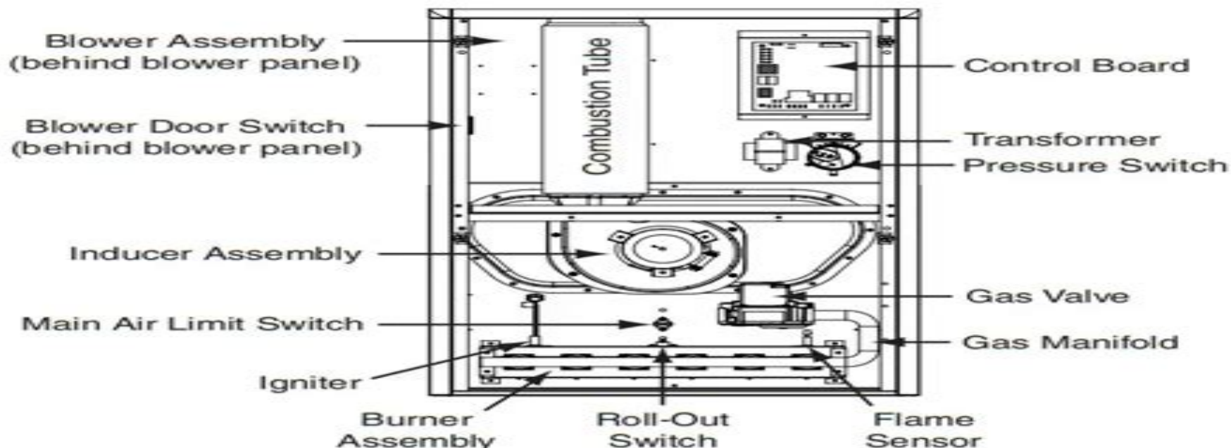
Downflow Gas Furnace
