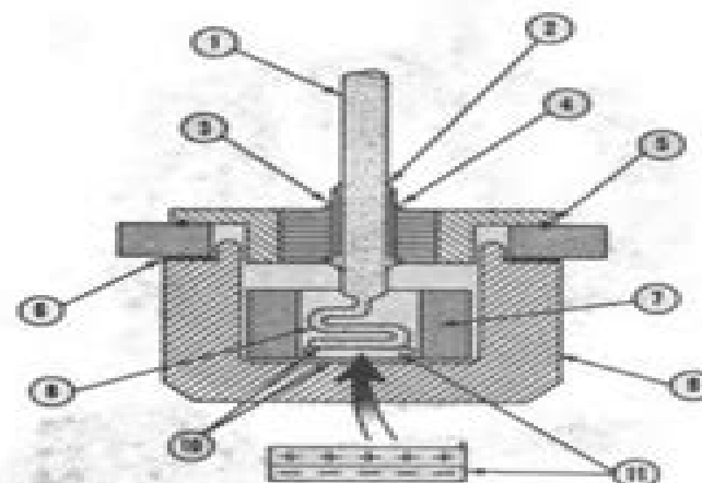
Figure 6 Diode Construction
