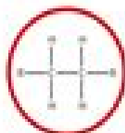
ALKANE
