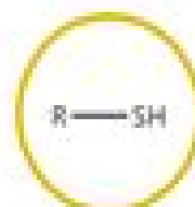
THIOL
