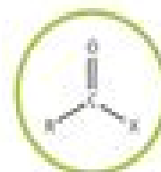
ACYL HALIDE
