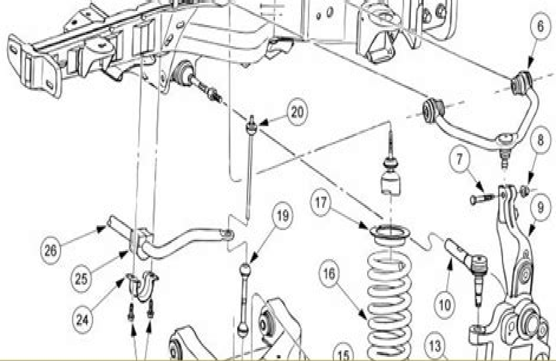
2wd Ford Ranger Front Suspension Diagram
