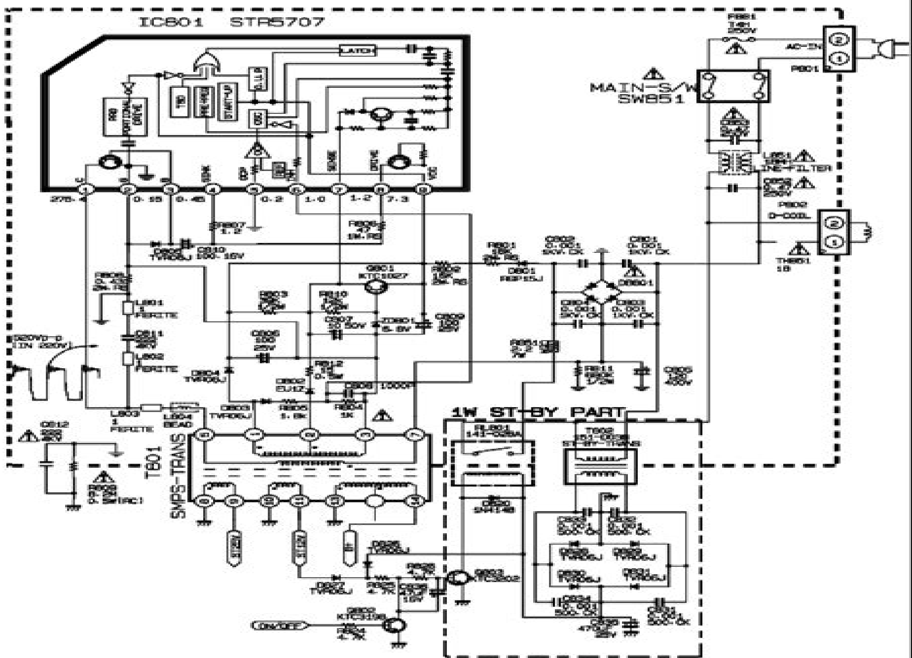
<FIG 1> STR-S5707 CIRCUIT DIAGRAM
