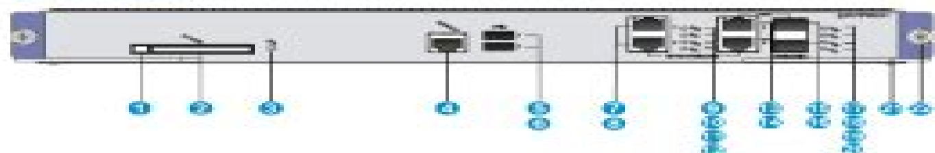
Figure 1 Front panel
