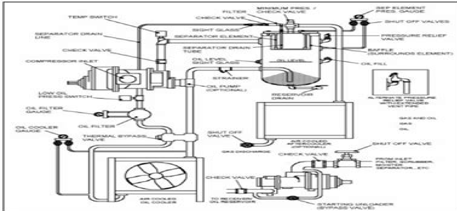
Figure 4 – Typical Basic Piping Diagram
