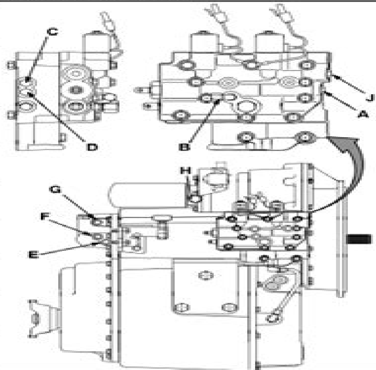
FIGURE 38. TRANSMISSION PRESSURES
