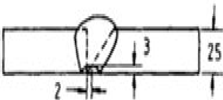
(a) Desired weld
