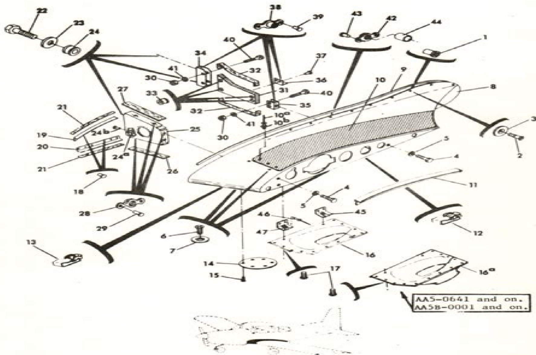
FIGURE 3. WING ROOT ASSEMBLY & INSTALLATION
